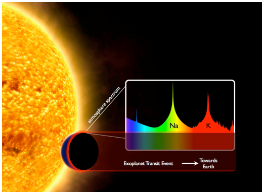
Figure 2: Spectroscopy of exoplanetary atmosphere -credit http://astro.ufl.edu
