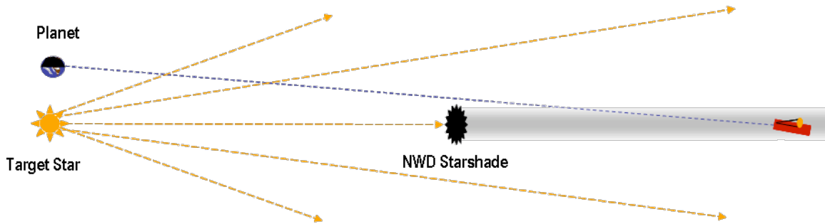
Figure 3: Design plan of the proposed Exoplanet Imager - New Worlds Observer - Credit: NWO team
