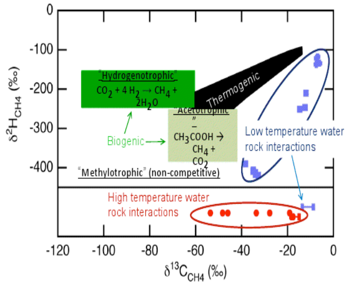
Figure 4: Classification of trends in H and C Isotopic fractionation Credit: Image courtesy of presentation by Dr. Bebout based off Allen, M. 2006
