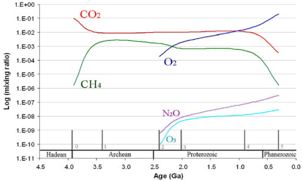
Figure 1: log scale amounts of atmospheric constituents over the history of Earth - Credit: Kaltenegger et al 2007
