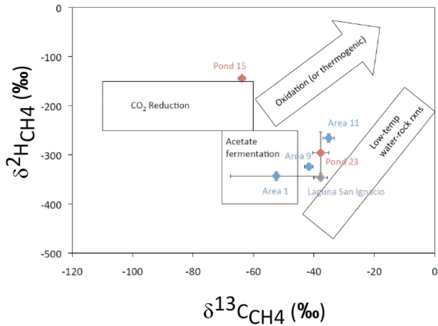
Figure 5: Methane isotopes from hypersaline sites – Image courtesy of Dr. Bebout and his research team
